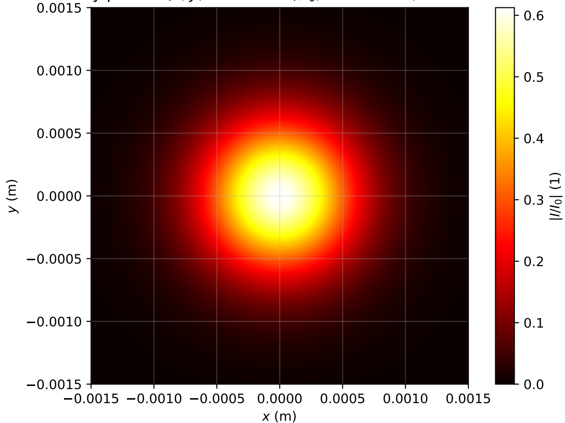
Intensity profile I(x, y, z = 2.149m)/I_0 , Pin=0.3Pcr, artificial time
